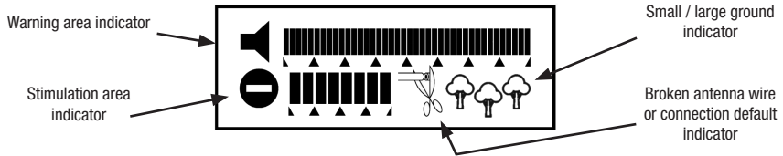
Diagram 2 – LCD screen
